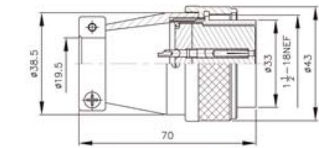
PLS-35-PF
