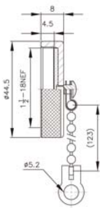
AMS25043-24A
