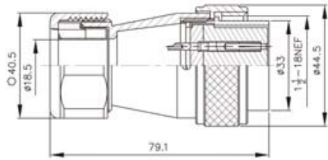
PLS-35-GPF3/4"
