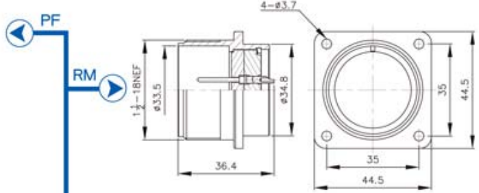
PLS-35-RM
